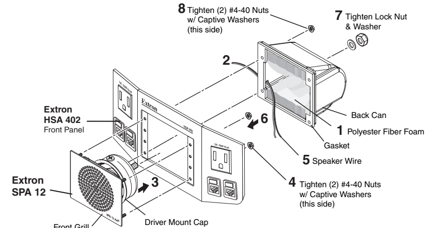
Figure 2 — Mounting the SPA 12 onto the HSA 402
