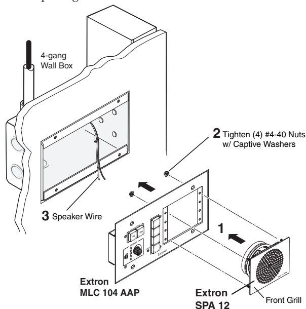
Figure 4 — Mounting the SPA 12 into an MLC 104
